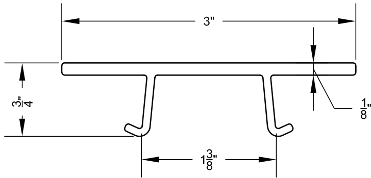
1 W-CLIP DETAIL SCALE: 1" = 1"
