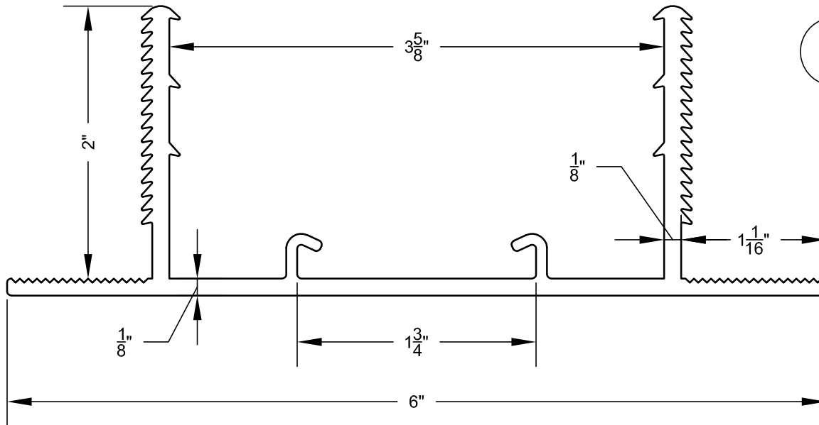
2 E-CHANNEL / E-BRIDGE DETAIL SCALE: 1" = 1"
